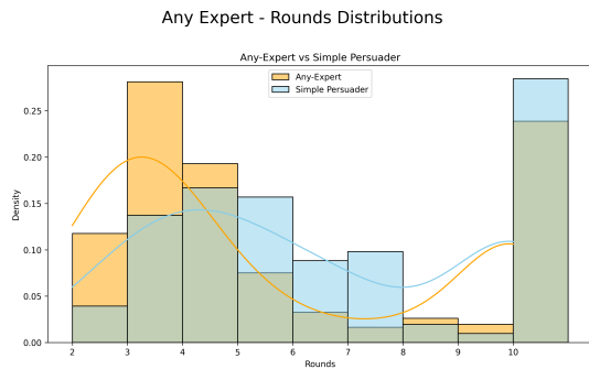
Figure 2: Distribution of debate rounds for expert persuaders (orange) versus baseline (blue). Mean rounds: 5.31 vs. 6.25 (Cohen’s d = -0.654 ).
