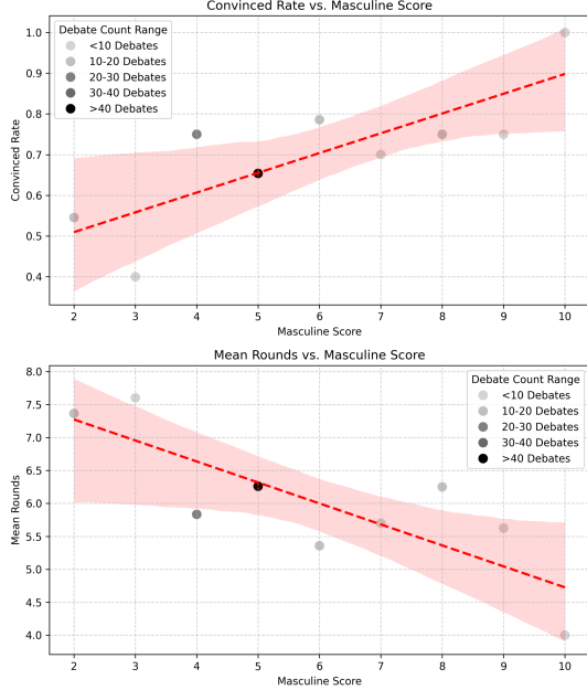
Figure 3: Relationship between topic masculinity score and debate outcomes for M→F configuration. Top: Convinced rate increases with masculinity score ( r = +0.66 ). Bottom: Mean rounds decrease with masculinity score ( r = -0.64 ), indicating faster resolution on masculine topics. Regression lines with 95% confidence intervals shown. Point colors indicate debate count per masculinity score bin.
